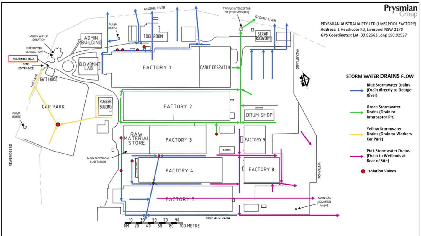
Figure 7-1: Stormwater Drains and Isolation Valves Layout
